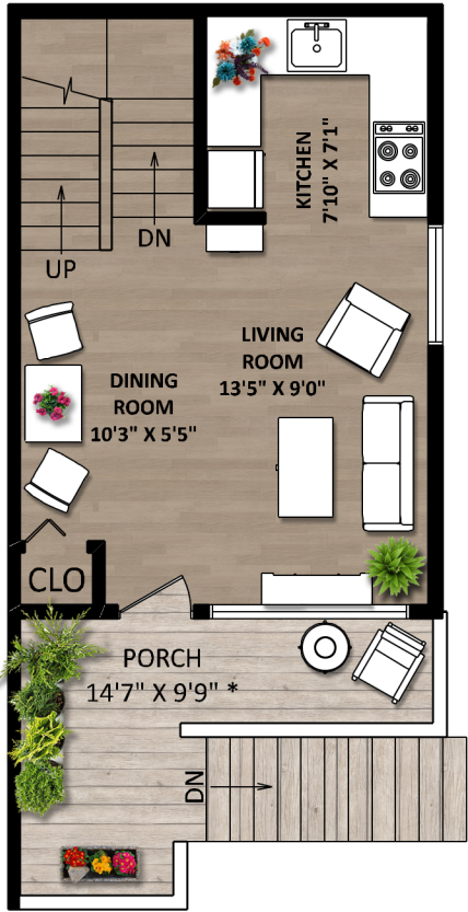
MAIN FLOOR: 323 SQ.FT.
